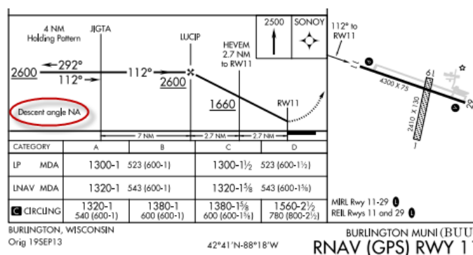
Figure 1: No Published Vertical Descent Angle (VDA) Example
