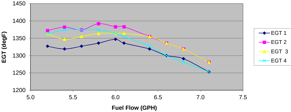
EGT vs. Fuel Flow 18.2" MAP, 2,300RPM 13,300' PressAlt
