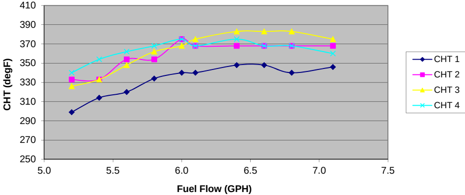
CHT vs. Fuel Flow 18.2" MAP, 2,300RPM 13,300' PressAlt
