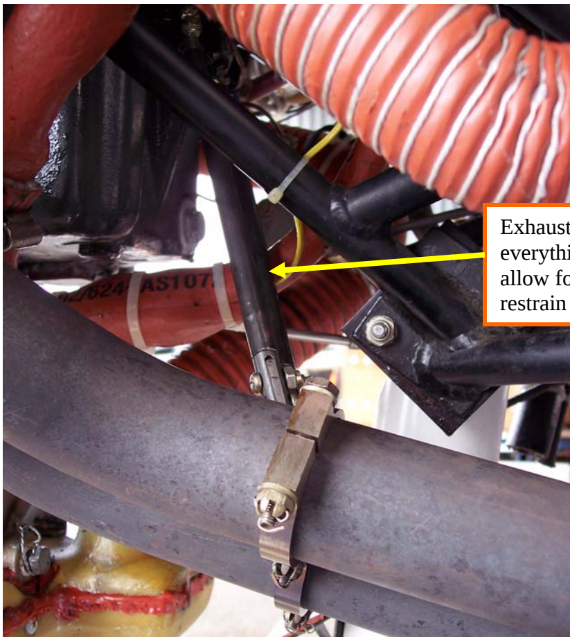
Stainless Steel bracket and bolts used to clamp exhaust pipes
