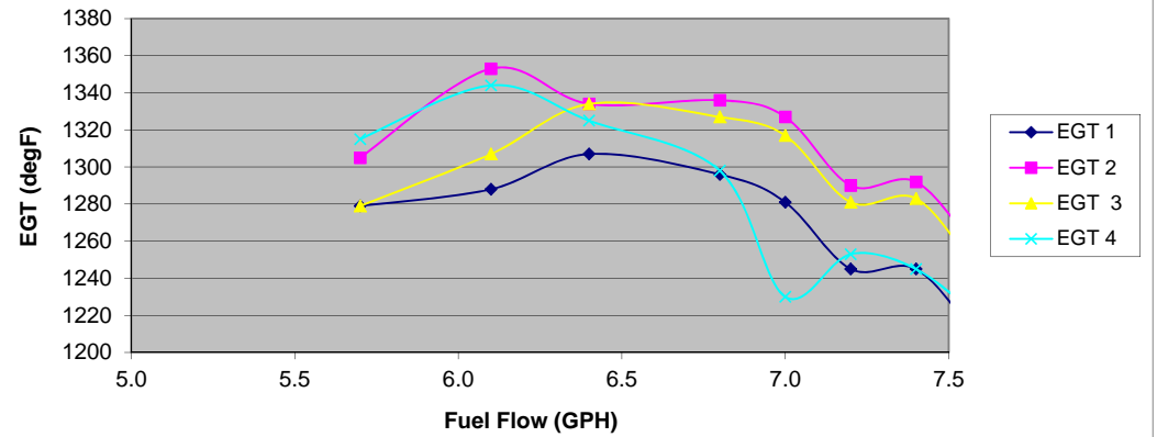
EGT vs. Fuel Flow 18.8" MAP, 2,300RPM 13,300' PressAlt
