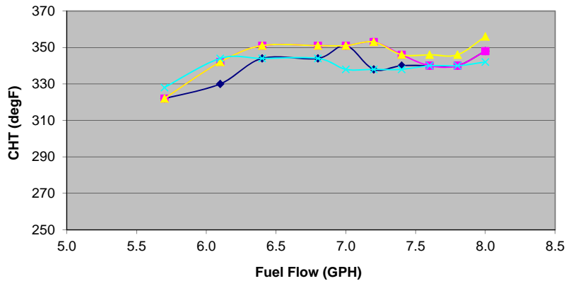
CHT vs. Fuel Flow 18.8" MAP, 2,300RPM 13,300' PressAlt
